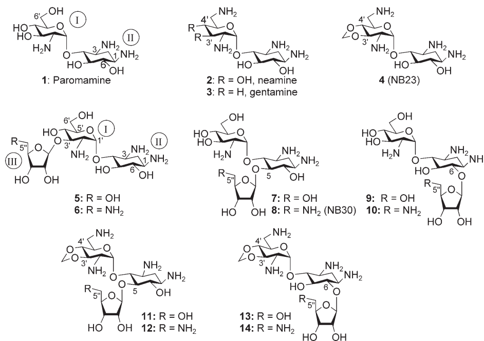
Figure 1. Sets of 2-DOS-containing pseudo-disaccharides (compounds 1–4 ) and pseudo-trisaccharides (compounds 5–14 ) that were tested for the tolerance toward the enzymatic addition of AHB moiety.
