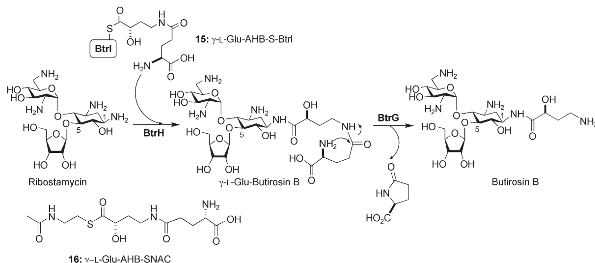
Scheme 1. Biosynthetic pathway for the conversion of ribostamycin to butirosin B.
