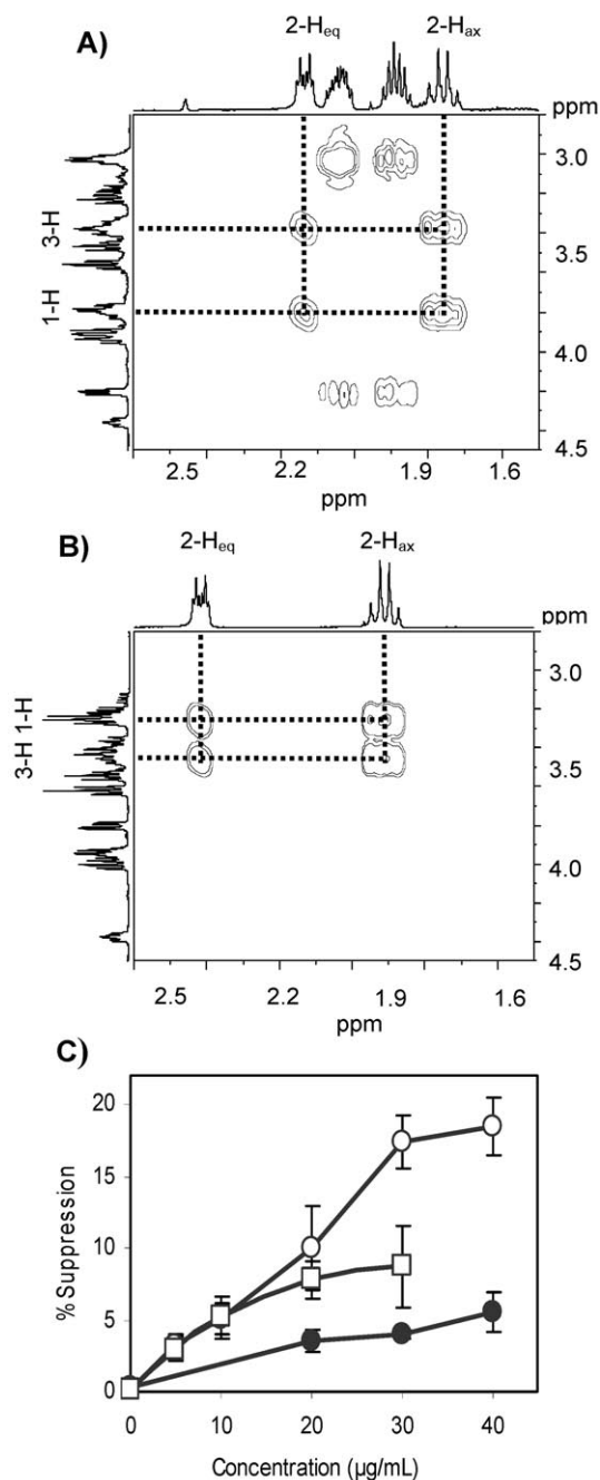
Figure 2. Partial 2D 1 H- 1 H COSY spectra of the chemoenzymatically produced N-1-AHB-4 ( A ) and of its parent compound 4 ( B ). The dashed lines show correlations between 2-H ax and 2-H eq protons with 1-H and 3-H protons of the 2-DOS ring, highlighting strong downfield shift of the 1-H proton in N-1-AHB-4 versus 1-H proton in the parent compound 4 . Panel C shows the levels of in vitro suppression of a TGA C nonsense mutation by compound N-1-AHB-8 (○), by compound 8 (●) and by natural drug paromomycin (□).
