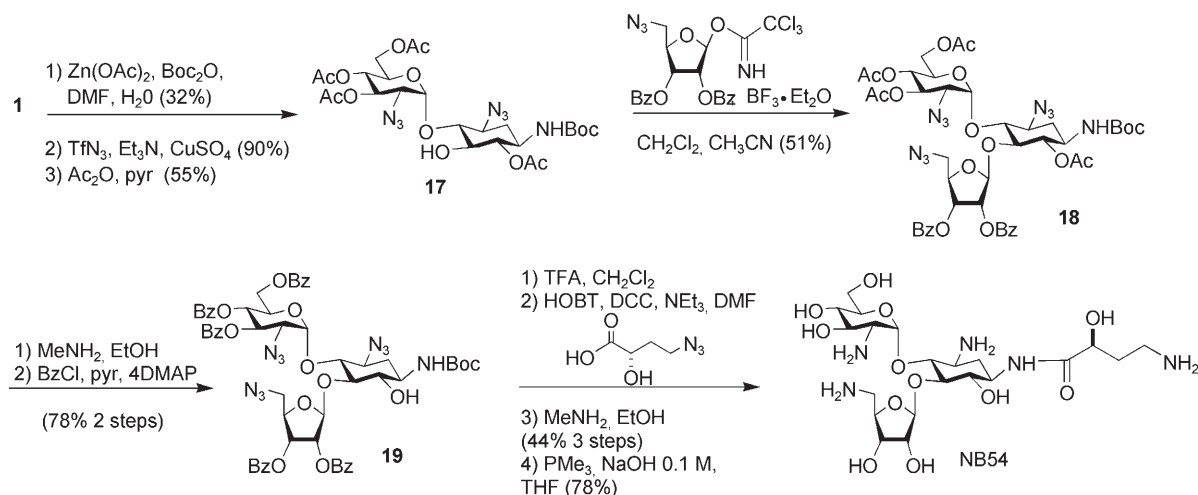
Scheme 2. Chemical transformation of paromamine 1 into NB54. [18]
